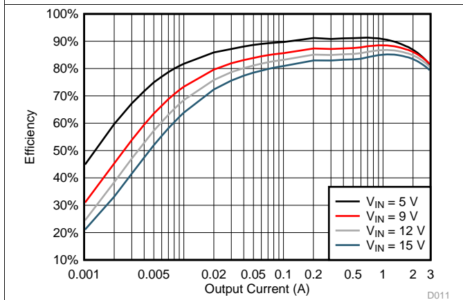
Figure 9. TPS563201 V_{OUT} = 1.05\text{ V} Efficiency, L = 2.2\text{ }\mu\text{H}
