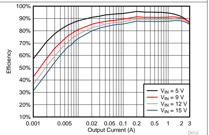
Figure 10. TPS563201 V_{OUT} = 1.5\text{ V} Efficiency, L = 2.2\text{ }\mu\text{H}
